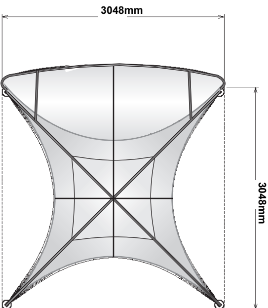
3m City B Dome Footprint Dimensions
